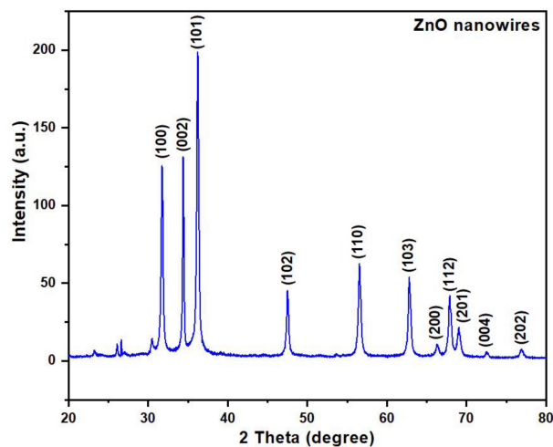
FIGURE 2 | XRD pattern of ZnO nanowires.
