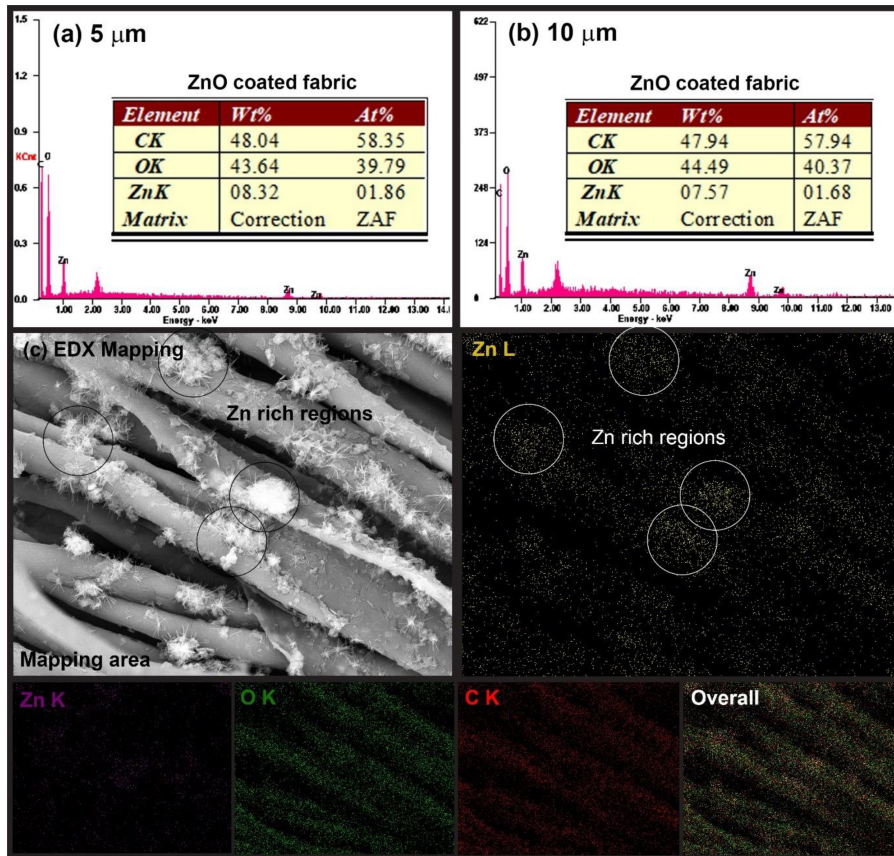
FIGURE 4 | EDX spectra of ZnO nanowires coated cotton fabric scanned at different areas (a) 5 μm, (b) 10 μm and (c) EDX mapping spectra of ZnO nanowires coated cotton fabric.
