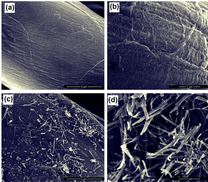
FIGURE 3 | FESEM images of uncoated (a, b) and coated (c, d) cotton fabric.
