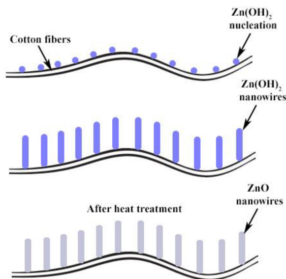
FIGURE 1 | Schematic explaining the formation of ZnO nanowires over cotton fibers.
